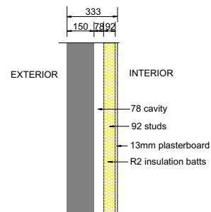
External Wall System 299 Sussex St Sydney
